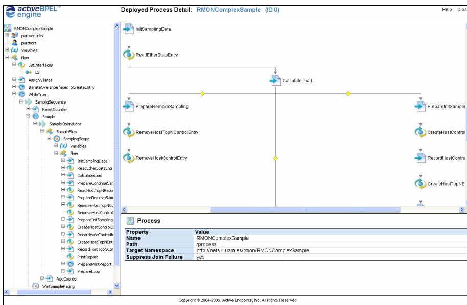
Fig. 4. Load-based Network Management process deployed in the ActiveBPEL Engine.
