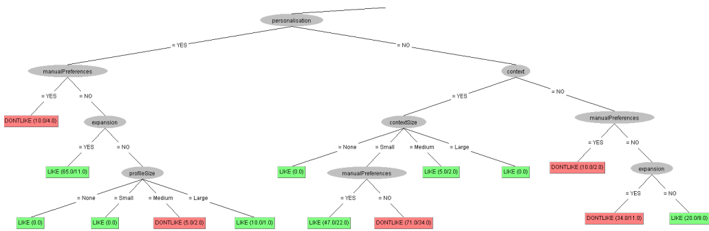
Fig. 4. Headlines branch in the first page and using all the available logs (general evaluation).
