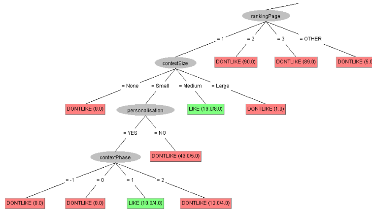
Fig. 6. World branch using context related logs (goal-based evaluation).
